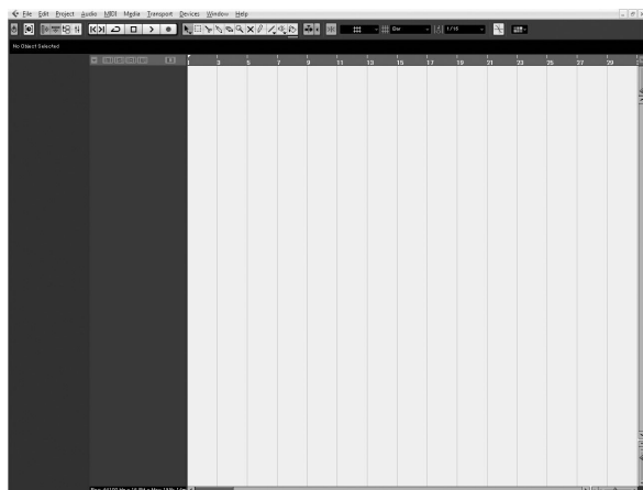
Project window
